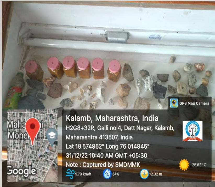
Rock Sample
